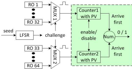
Figure 6: An implementation of RO-PUF.
