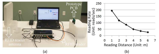
Figure 10: (a) Experimental setup for evaluating RF performance and (b) RFID reading efficiency.
