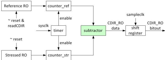
Figure 5: A RO-based CDIR sensor.
