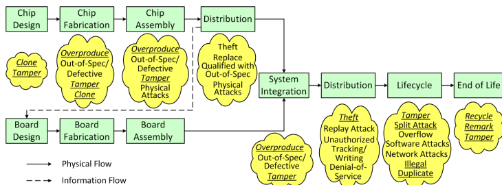
Figure 1: Electronic components and systems supply chain vulnerabilities.
