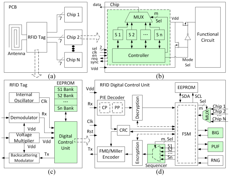
Figure 2: CST system: (a) A PCB with an RFID tag connected to different chips, (b) Internal structure of a chip with various sensors, (c) Internal structure of an RFID tag, and (d) Internal structure of the digital control unit in an RFID tag.
