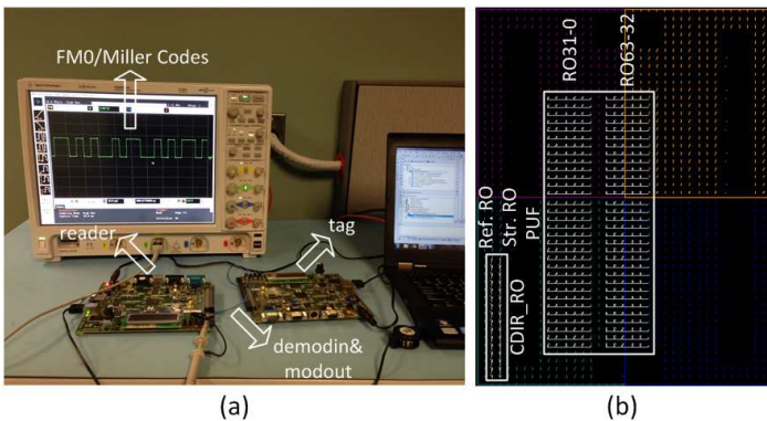
Figure 8: (a) Experimental setup and (b) FPGA layout of the RFID tag digital part.
